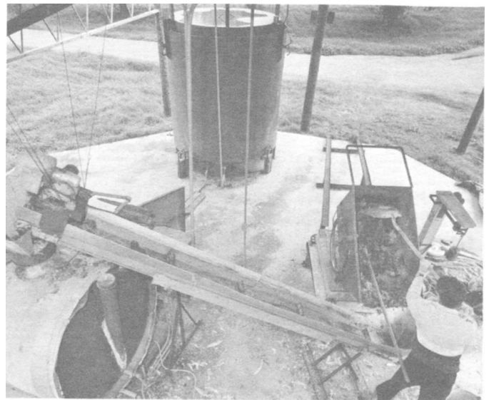
Loading poultry wastes into a methane generator.
